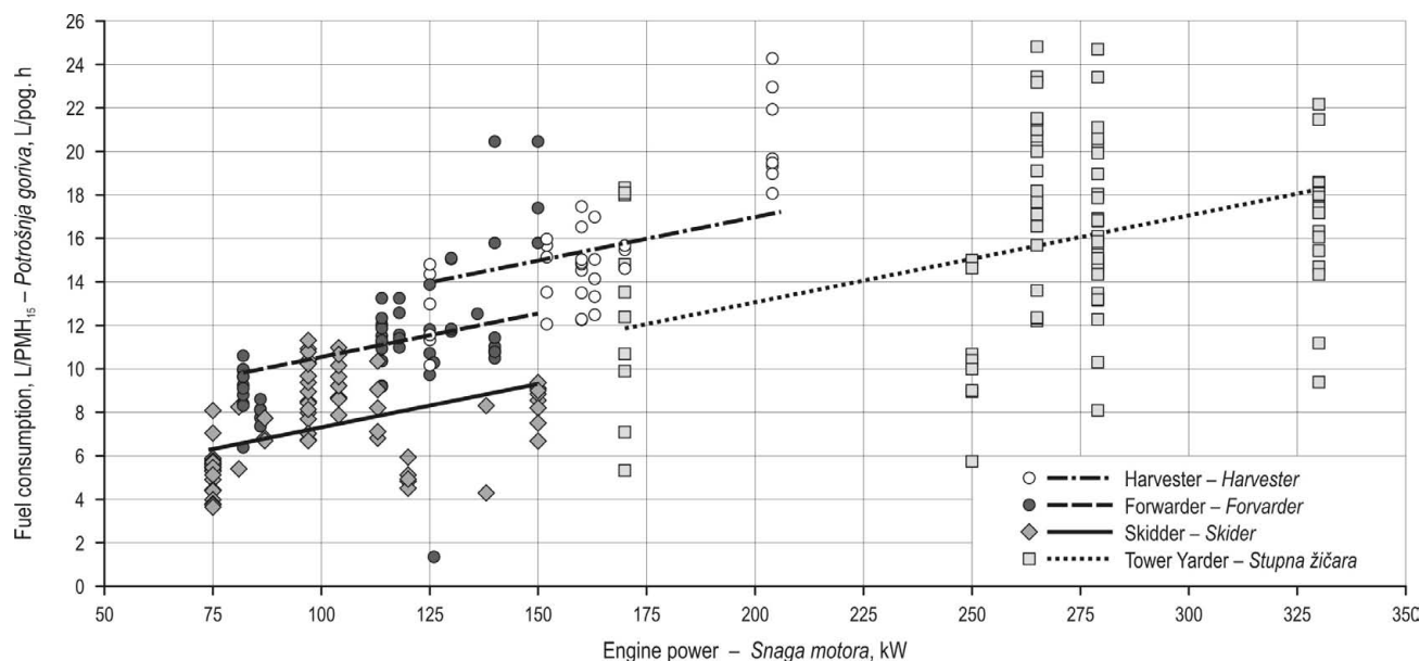
Fig. 1 Observed fuel consumption and the model based estimates of different forest machinery
