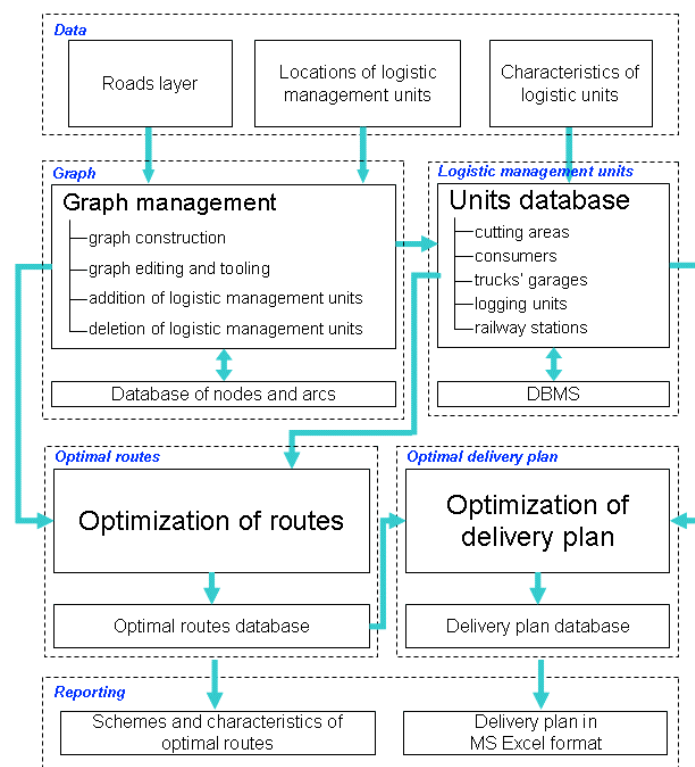
Figure 2. An overview of the DSS structure
