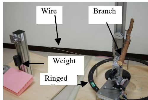
Figure 10. Experimental environment of circular orbit cut
